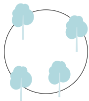
FIG. 1 – SEPARATED Trees are widely spaced and crowns do not touch or overlap
